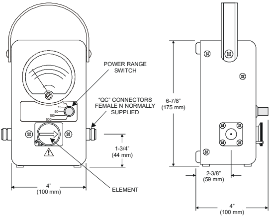
Figure 1 Bird 4304A Thruline Wattmeter Outline Drawing
