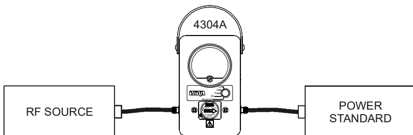
Figure 10 Calibrating the 4304A-1 Element
