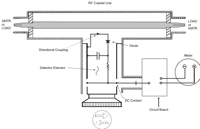
Figure 2 Thruline Wattmeter Schematic
